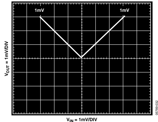
Figure 32. Absolute Value Circuit Performance (Input Signal = 0.05 Hz)
